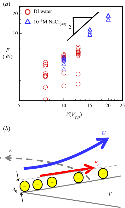
Figure 8. (a) Plot of the measured force F = 4\pi\eta Ur against the applied voltage V for AC electro-osmotic impinging flow in deionized water (at 80 kHz) and 1 mM NaCl solution (at 100 kHz), which shows F \propto V^2 . Multiple data points at a given value of V are the data points taken from different values of r shown in figure 3(b). (b) Illustration of the flow mechanism, driven by an electric force within the double layer.
